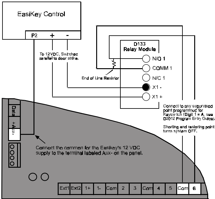
Figure 13: Keyswitch
