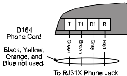
Figure 7: Phone Cord
